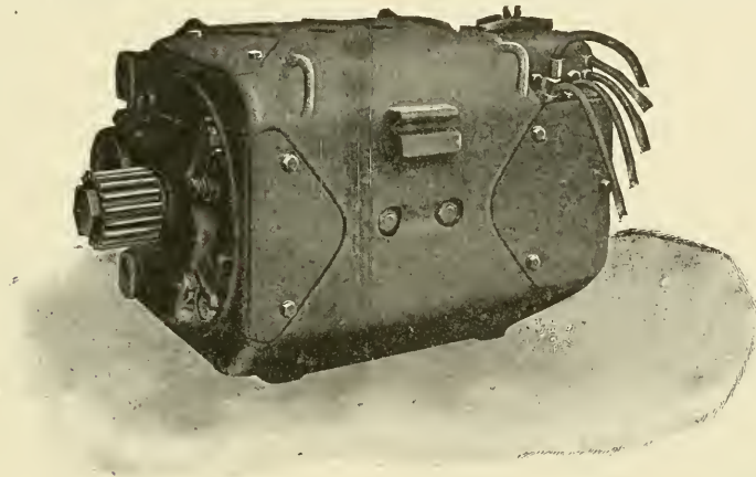
Fig. 43. Box Frame Motor—General Electric Company
